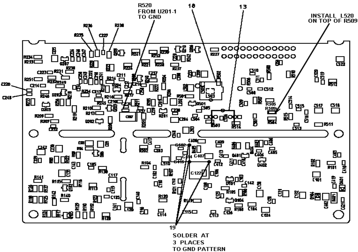
VIEW FROM SOLDER SIDE
